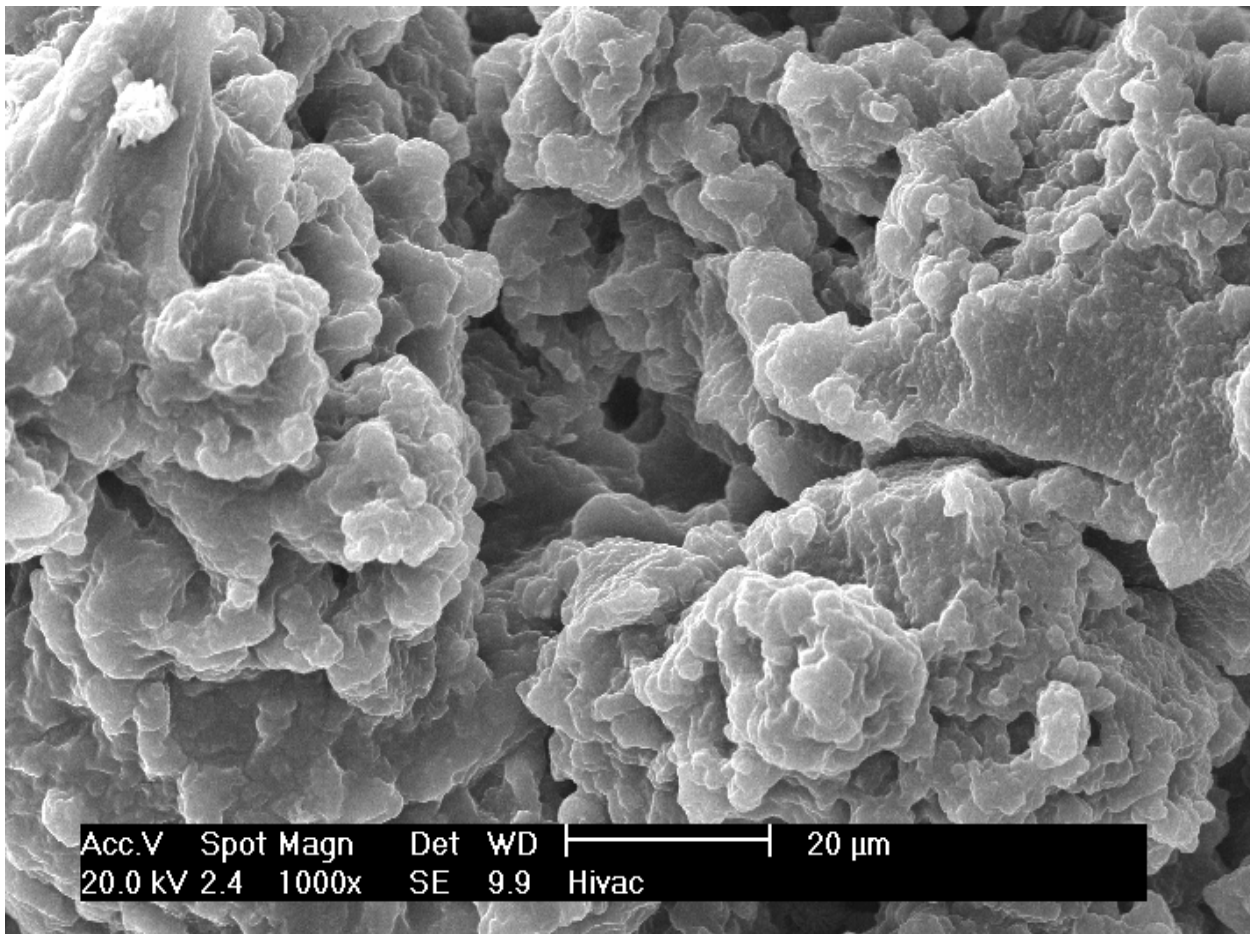
PIPE.RUBBER in Internal Olefin at 250F. 20 micron scale
